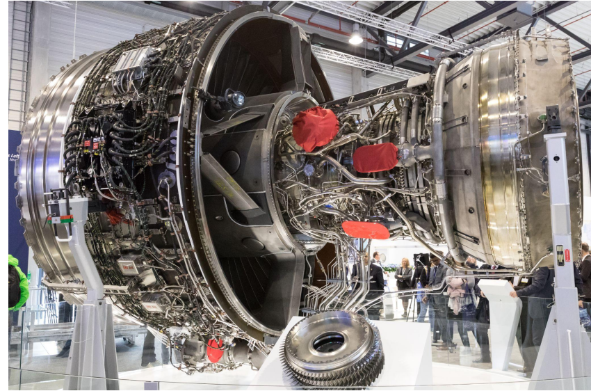
The inside of a Rolls-Royce Trent XWB Turbofan engine.
